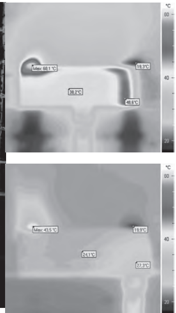
Thermography Cool Body technology (picture: CeraTherm) hinders the overheating of the fitting body in the Ideal Standard thermostats, preventing burns.
